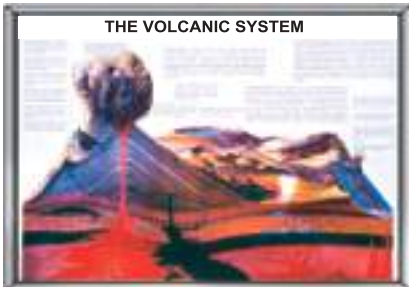
RRC-07 THE VOLCANIC SYSTEM
