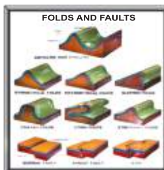
RRC-14 FOLDS & FAULTS
