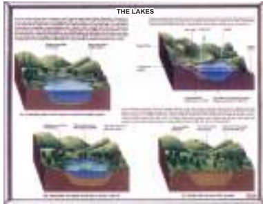
RRC-16 THE LAKES
