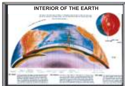
RRC-01 INTERIOR OF EARTH
