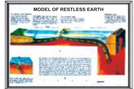
RRC-09 MODEL OF RESTLESS EARTH
